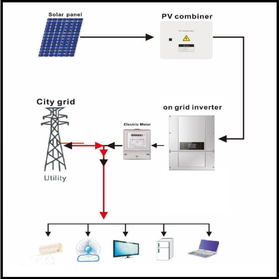
On Grid System
